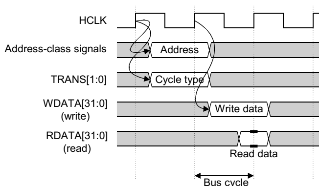
Figure 6-3 Simple memory cycle
